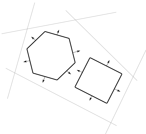
Figure 202: Finding the axes for the SAT (2/2)
